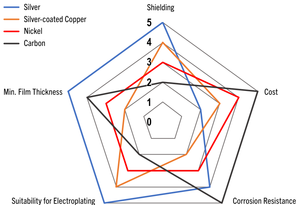
Graph 2. Performance comparison of conductive paints based the filler type. 5 represents the highest performance and 1 represents the lowest performance.
